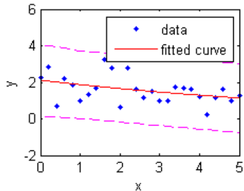
Simultaneous functional bounds
