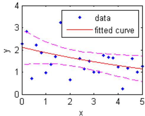
Simultaneous functional bounds
